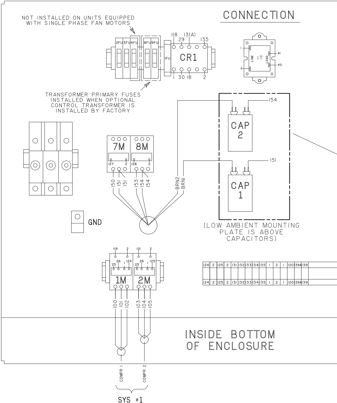
FIGURE 24 - CONNECTION WIRING, SINGLE CIRCUIT
