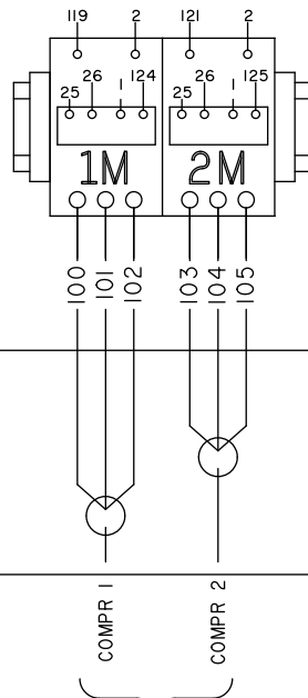
FIGURE 27 - CONNECTION WIRING, SINGLE CIRCUIT
