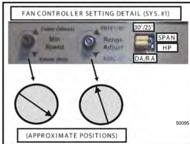
FIGURE 47 - POTENTIOMETER SETTINGS
