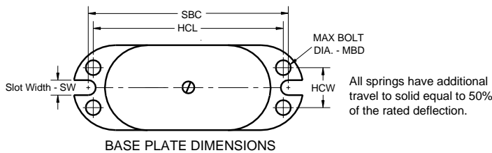
BASE PLATE DIMENSIONS
