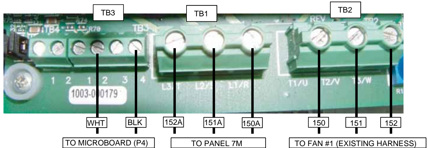
FIGURE 53 - INVERTER WIRING
