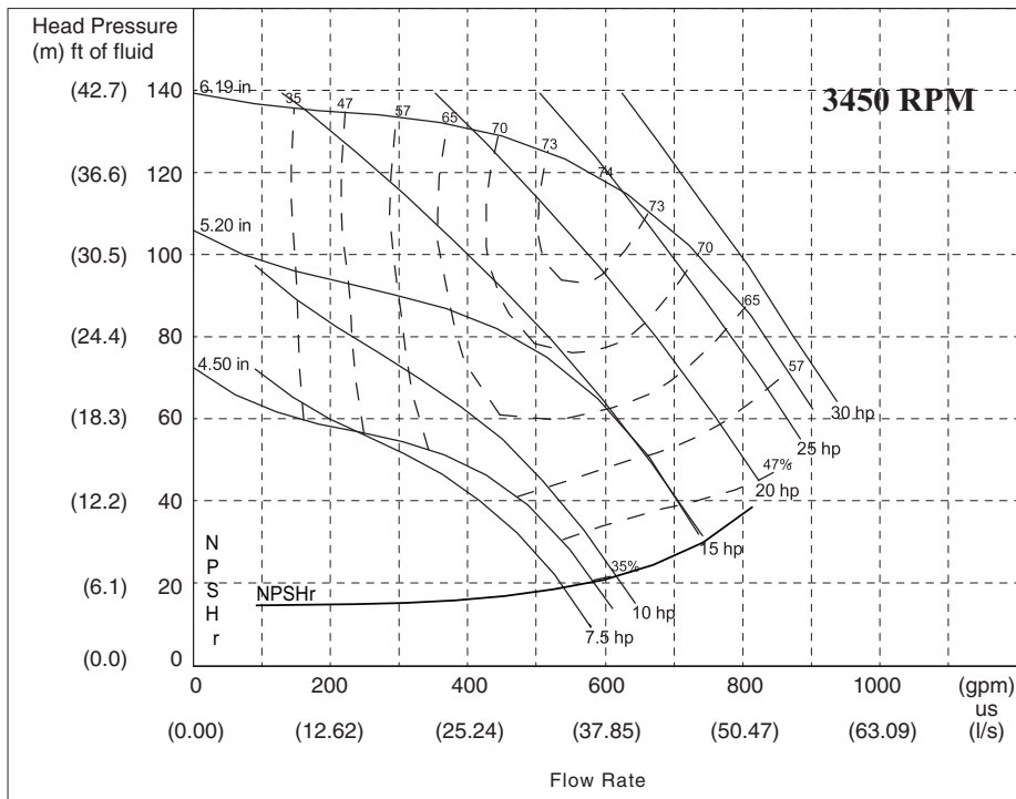
PUMP CURVE IVB FOR HYDRONIC PACKAGE SINGLE PUMP (Fresh Water)
