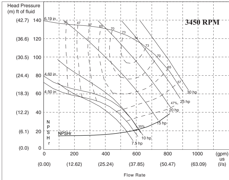
PUMP CURVE IVA FOR HYDRONIC PACKAGE SINGLE PUMP (Fresh Water)
